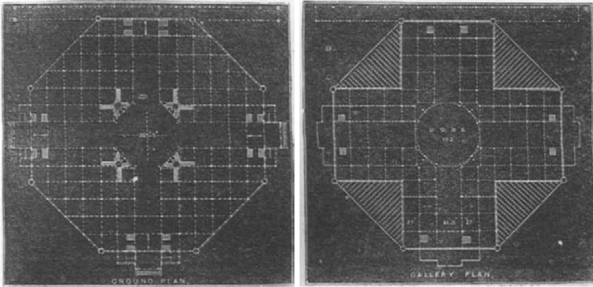
Fig. 35. Charles Gildemeister and George J. B. Carstensen, architects, New York Crystal Palace, Ground and Gallery Plans , 1852. Lithograph, from Appleton's Mechanics' Magazine 3 (February 1853), pp. 35–36. Courtesy of the American Antiquarian Society, Worcester, Massachusetts
