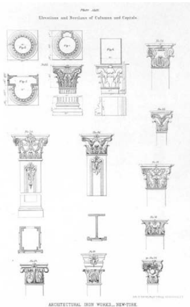
Fig. 18. Cast-Iron Components . Lithograph, from Badger's Architectural Iron Work Catalogue (New York: Baker and Godwin, 1865), pl. 49. Cooper-Hewitt, National Design Museum, Smithsonian Institution, Washington, D.C.
