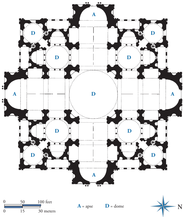
17-22 DONATO D'ANGELO BRAMANTE, plan for Saint Peter's, Vatican City, Rome, Italy, 1505.
