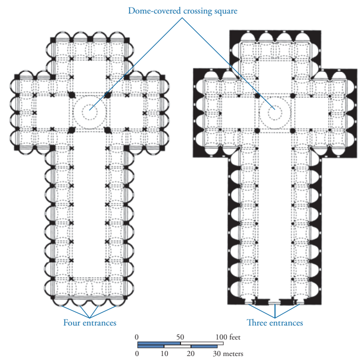
16-33 FILIPPO BRUNELLESCHI, early plan ( left ) and plan as constructed ( right ) of Santo Spirito, Florence, Italy, designed 1434–1436; begun 1446.
