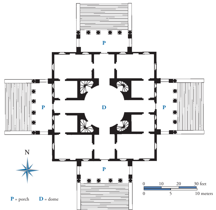
17-29 ANDREA PALLADIO, plan of the Villa Rotonda (formerly Villa Capra), near Vicenza, Italy, ca. 1550–1570.
