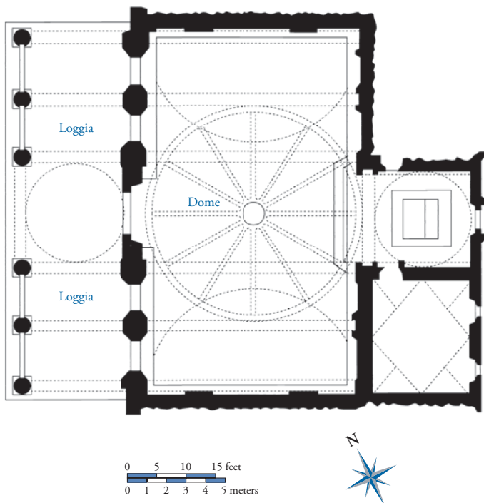
16-35 FILIPPO BRUNELLESCHI, plan of the Pazzi Chapel, Santa Croce, Florence, Italy, begun 1433.
