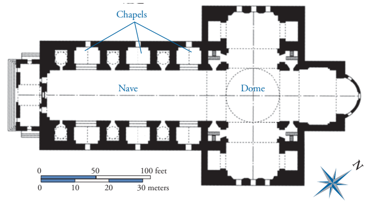
16-46 LEON BATTISTA ALBERTI, plan of Sant'Andrea, Mantua, Italy, designed 1470, begun 1472.
