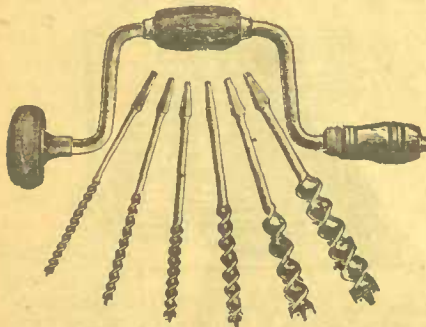
Tool set No. 32—Carpenters' Medium Brace and one Auger Bit each, \frac{1}{4} , \frac{5}{16} , \frac{3}{8} , \frac{1}{2} , \frac{3}{4} and 1 inch. The bits are in a strong cottonade roll, each bit in a division by itself (same as in our bit set No. 29). This tool set No. 32 is an exceedingly handy set. The sizes of bits are all good. Price, per set, only $1.75, postage 50c extra.
