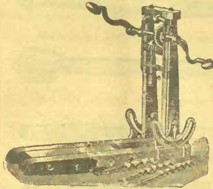
Improved Boring Machines Carpenters' and Framers' Boring Machines, best varnished hardwood frame and base, will bore straight or at any angle, with angle indicator; price, without augers, $5.50.
