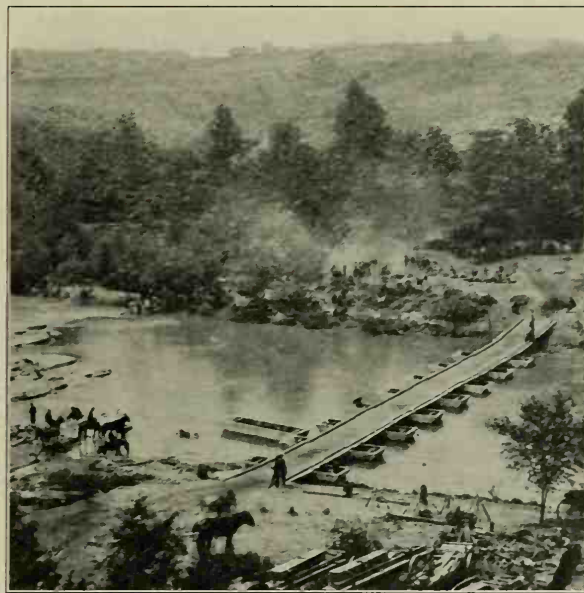
CANVAS PONTOON BRIDGE, NORTH ANNA RIVER
