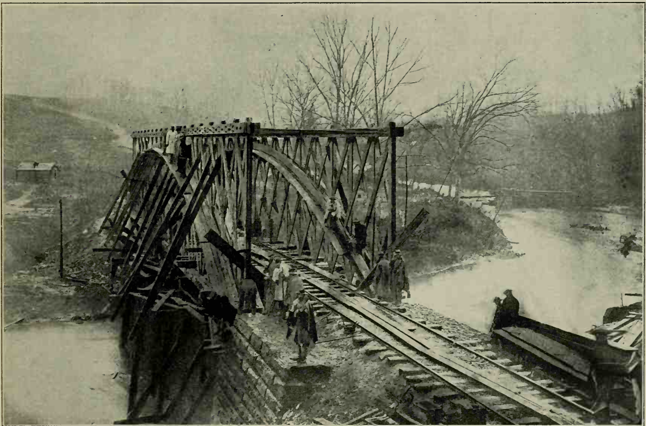
REINFORCED WITH TRUSSES—TRANSFORMED INTO A STANDARD BRIDGE
