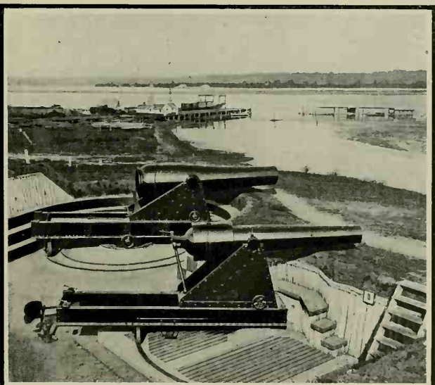
AN 8-INCH PARROTT AND A RODMAN GUN
