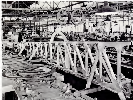
DURALUMIN WING SPAR FOR THE ATLANTIC CLIPPER IS 53 FT. LONG
