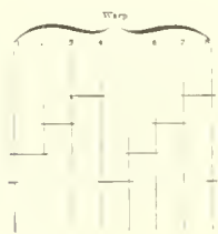
FIG. 133. Diagram Showing Arrangement of Threads of the Warp in the Healds and on the Rod.
