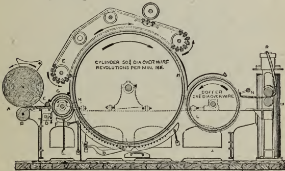
COTTON CARD
