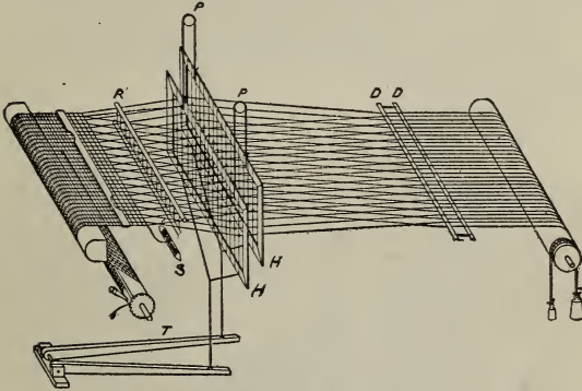
DIAGRAM OF THE WORKING PARTS OF A LOOM.
