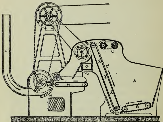
COTTON OPENER AND PICKER
