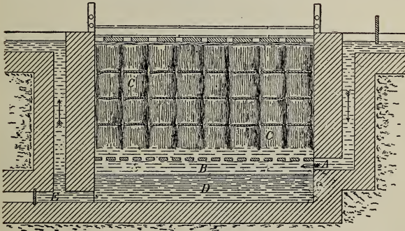
RETTING TANK
