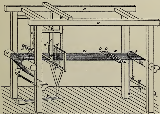
DIAGRAM OF A HAND LOOM
